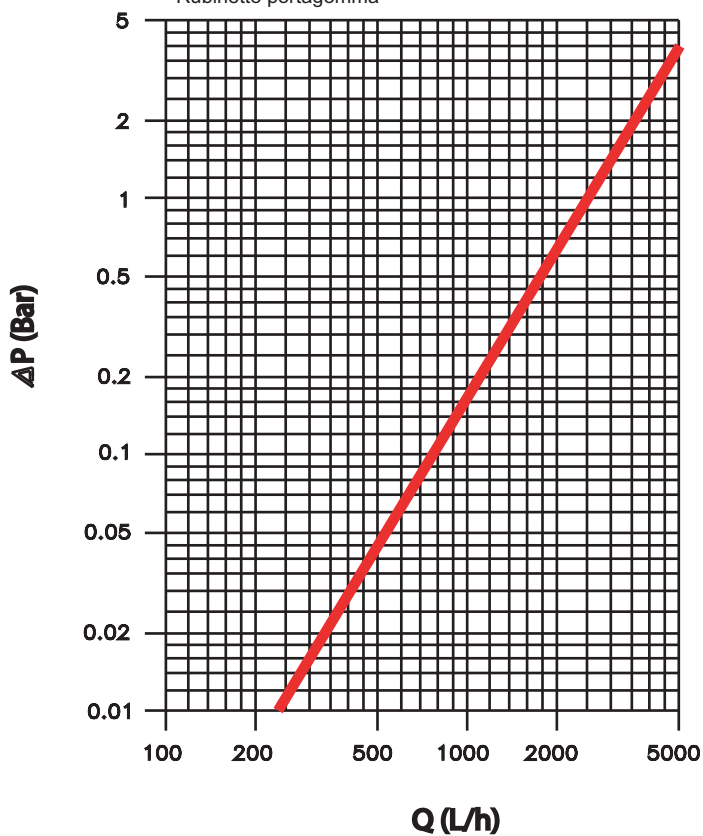
Art. 200---S--0 Rubinetto portagomma
